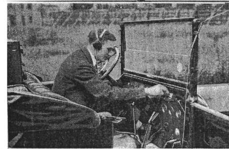
By Using the Telephone Transmitter of the Automobile Radio Set as a Telegraphic Sender, Ranges Up to 40 Miles Are Possible with the Portable Antenna
